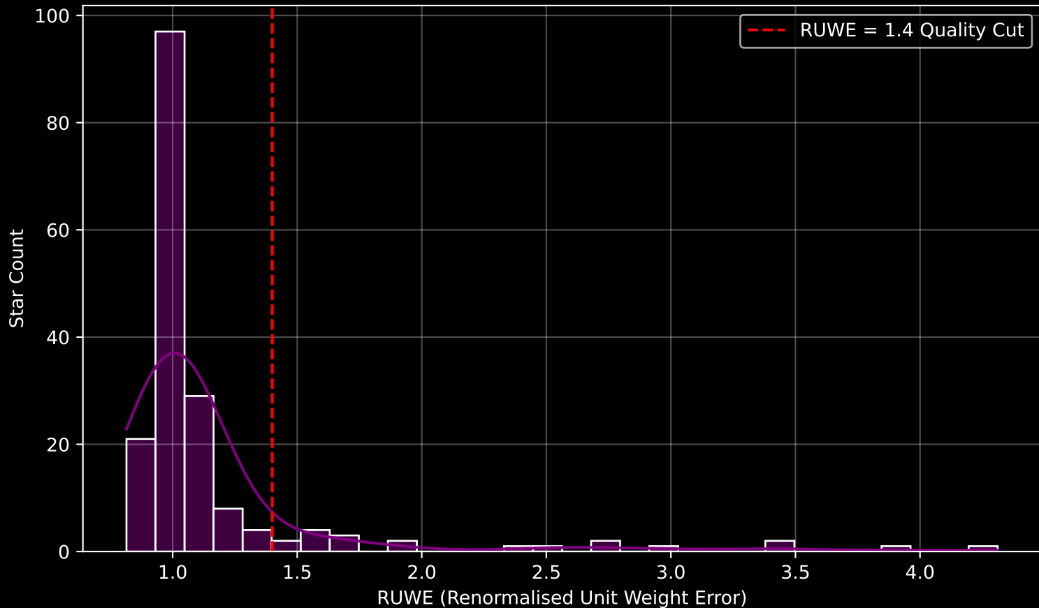
GAPOGEE DR17 Field [080+60] RUWE Distribution (n= 179)
